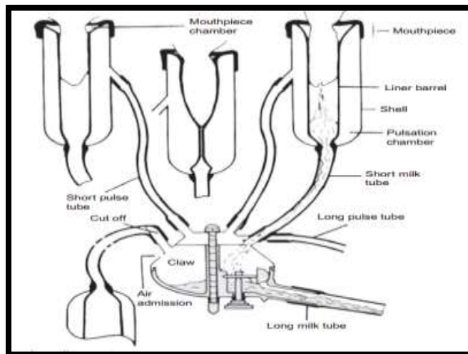
Fig. 5: Milking unit (Reinemann, 2013)
